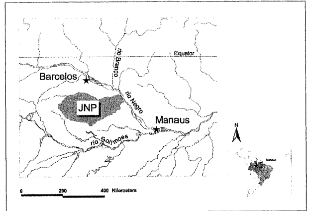
Figure 1. Location of Jaú National Park in Central Amazonia.
